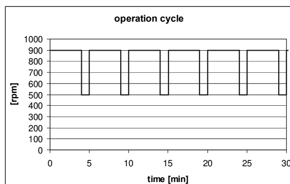
Figure 5: Operation Cycle 900/500*
