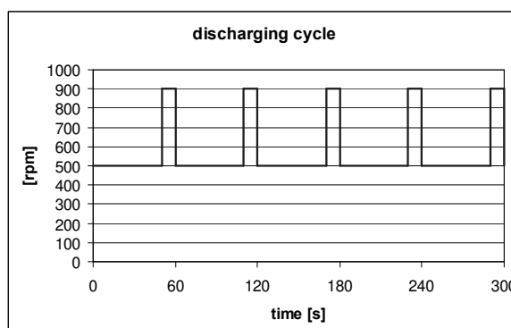
Figure 6: Discharging Cycle 500/900**
